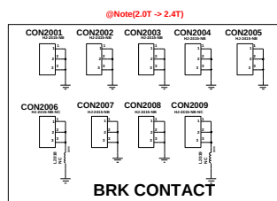
BRK CONTACT
